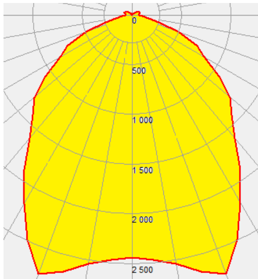
3F BETA A3F 2x91 LED VS With Wide Reflector
